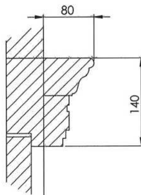
detail rampy
